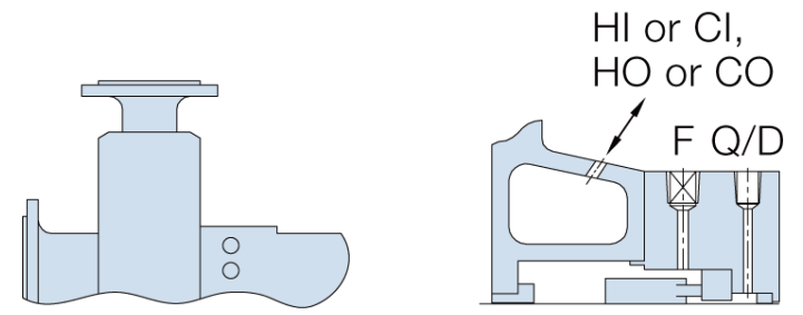
Plan 02 Dead End with Seal Gland Cooling
